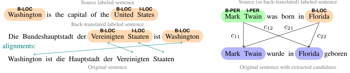
(a) Compute word-to-word alignments between back-translated and original sentences (b) Matching of extracted target candidates with source entities
