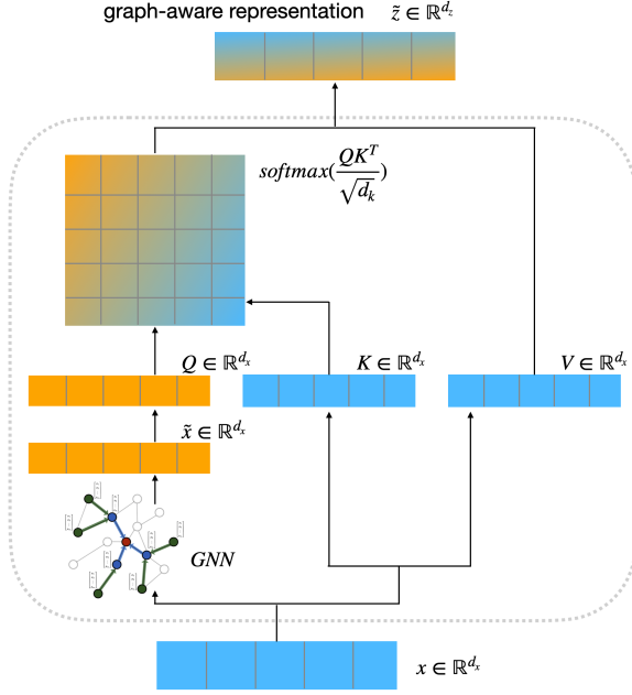
Figure 2: The architecture of GraSAGE. The text embedding x is fed into a GNN along with the edge index derived from the hierarchical graph structure. This process generates a graph embedding \tilde{x} , which subsequently induces the Q vector. The Q vector then guides the self-attention mechanism to produce a graph-aware representation \tilde{z} . The visualization of GNN is taken from GraphSAGE (Hamilton et al., 2017).
