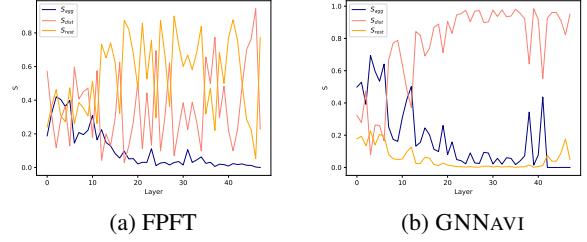
Figure 7: Comparison of information flow between FPFT and GNNNAVI for SST-2. Both models are trained with 5 training examples per class.
