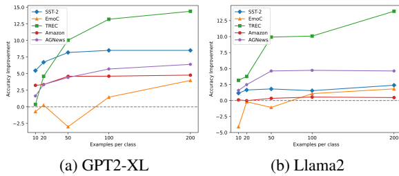
Figure 4: The improvement gained by adding training examples for GNNavi-SAGE, compared to using 5 training examples per class.
